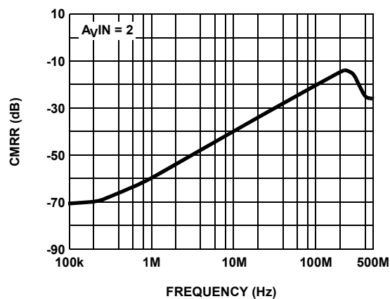
FIGURE 23. CMRR
