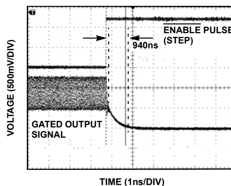
FIGURE 32. DISABLE TIME
