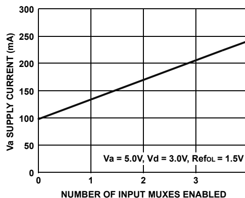
FIGURE 36. POWER SUPPLY CURRENT AS FUNCTION OF INPUT MUXES ENABLED (ALL OUTPUT MUXES DISABLED)
