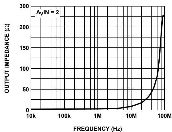
FIGURE 24. OUTPUT IMPEDANCE
