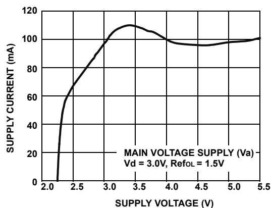
FIGURE 38. SUPPLY CURRENT VERSUS SUPPLY VOLTAGE BASE LINE IDLE (ALL INPUTS AND OUTPUTS DISABLED)
