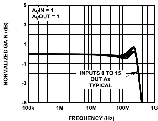
FIGURE 5. GAIN vs FREQUENCY FOR VARIOUS NON-INVERTING INPUTS
