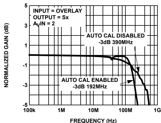
FIGURE 13. GAIN vs FREQUENCY FOR Sx CHANNEL FUNCTIONS
