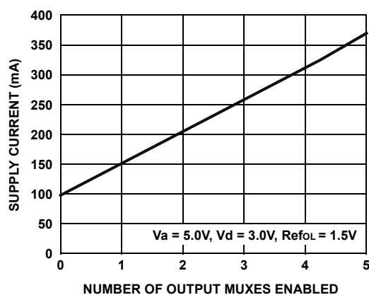
FIGURE 33. POWER SUPPLY CURRENT AS FUNCTION OF OUTPUT MUXES ENABLED - ALL INPUT MUXES DISABLED
