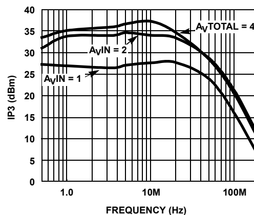
FIGURE 40. THIRD-ORDER INTERCEPT POINT vs FREQUENCY BLUE CHANNEL
