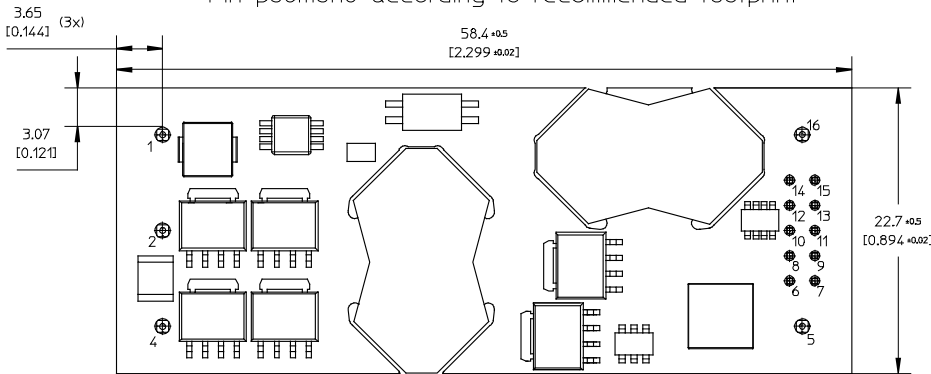
RECOMMENDED FOOTPRINT - TOP VIEW
