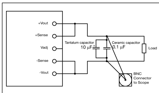
Output ripple and noise test setup
