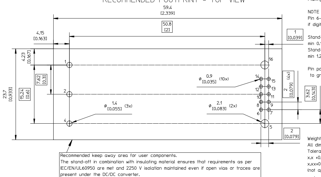
RECOMMENDED FOOTPRINT - TOP VIEW
