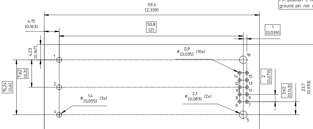
RECOMMENDED FOOTPRINT - TOP VIEW
