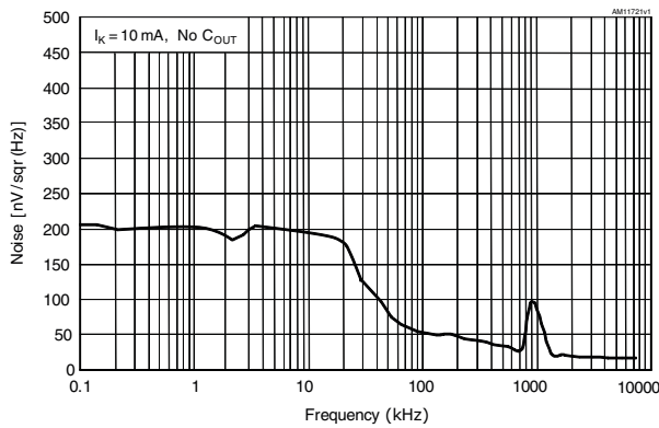
Figure 10. Wideband noise
