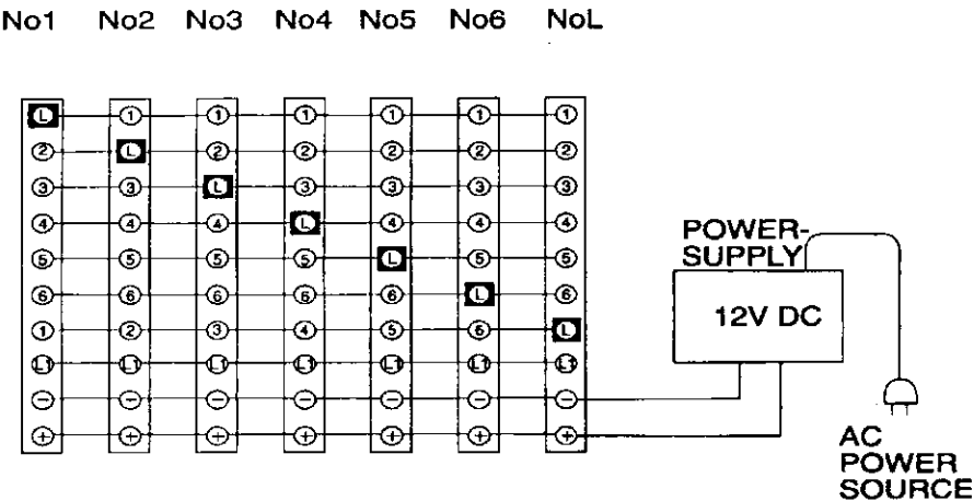
Figure 3. CM-206M Communications Network.
