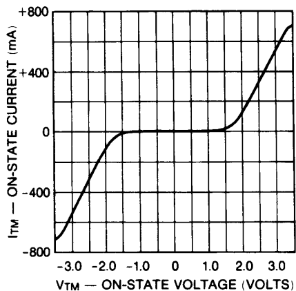
Fig. 1. On-State Characteristics
