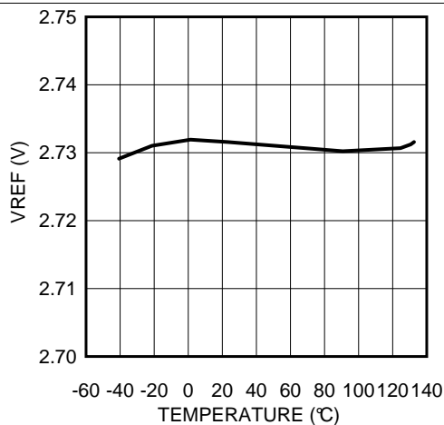
Figure 20. Reference Voltage
