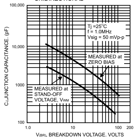
FIG.6- TYPICAL JUNCTION CAPACITANCE UNIDIRECTIONAL
