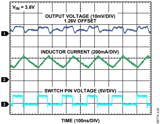
Figure 19. Standard Operation
