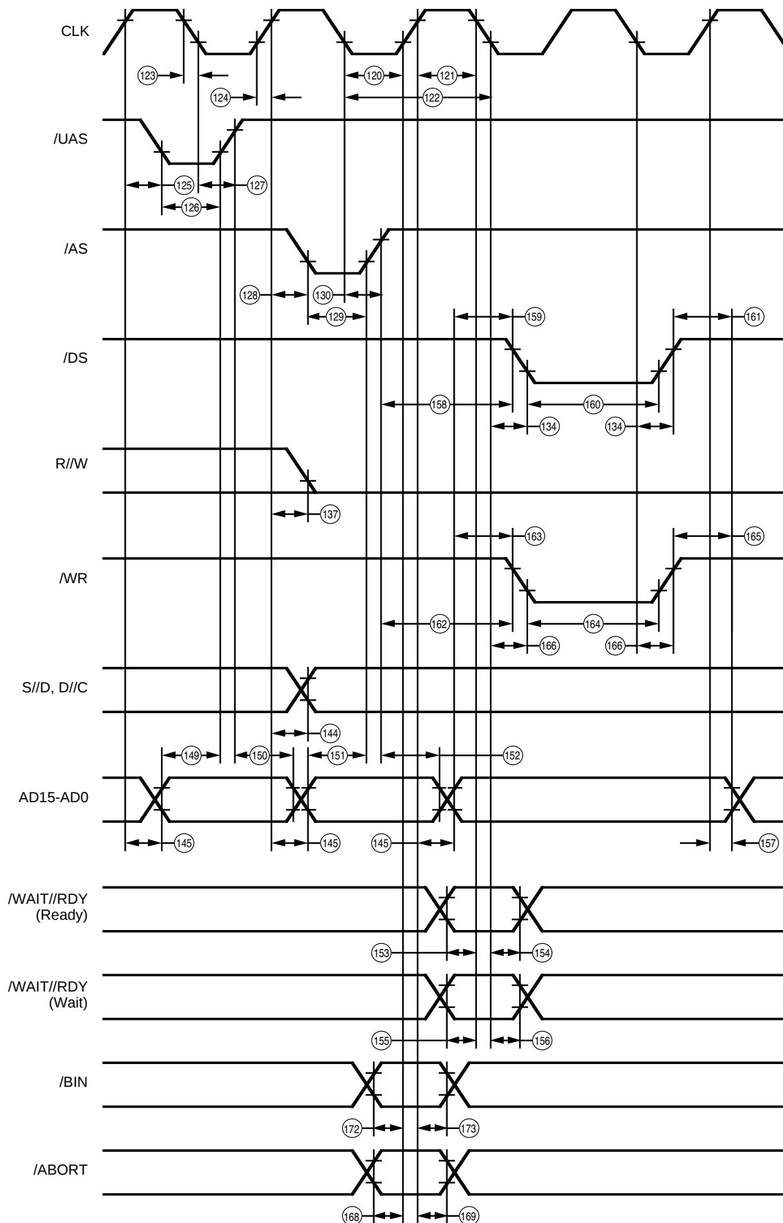
Figure 103. Memory Write
