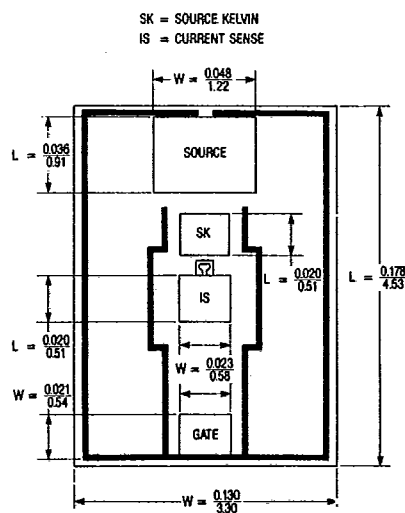
HEXSense-3: 60V, N-CHANNEL
