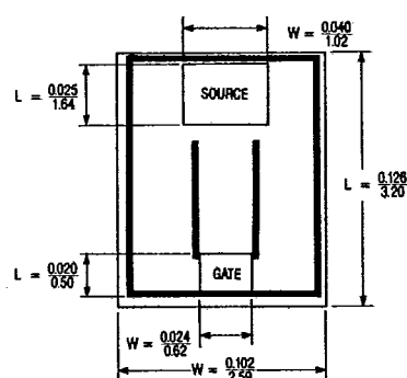
HEX-2: -60V, P-CHANNEL
