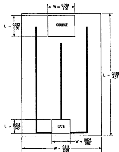
HEX-3: -100V, P-CHANNEL
