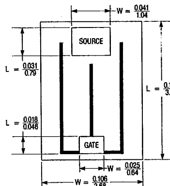
HEX-3: 100V, N-CHANNEL LOGIC LEVEL: HEX-3: 100V, N-CHANNEL
