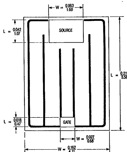
HEX-4: 200V & 250V, N-CHANNEL
