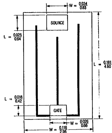
HEX-3: 200V & 250V, N-CHANNEL
