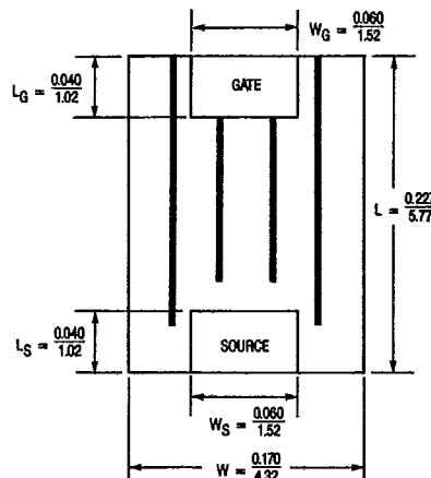
HEX-4: -200V, P-CHANNEL GEN I
