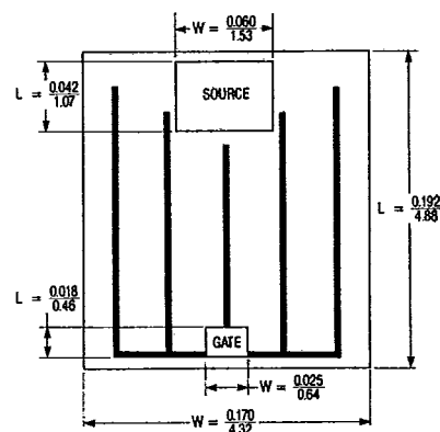
HEX-4: 100V, N-CHANNEL LOGIC LEVEL: HEX-4: 100V, N-CHANNEL
