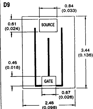
HEX-2: 400V & 500V N-CHANNEL
