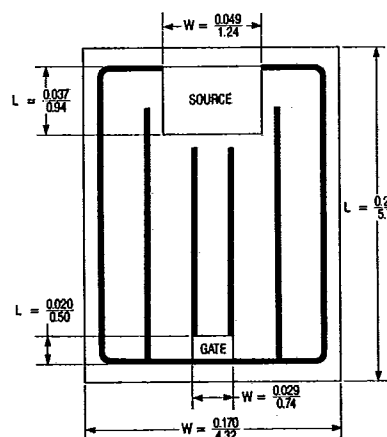
HEX-4: 400V, 500V, & 600V, N-CHANNEL
