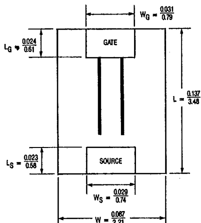
HEX-2: -200V, P-CHANNEL GEN I
