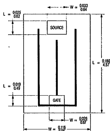
HEX-3: 400V, 500V, & 600V, N-CHANNEL
