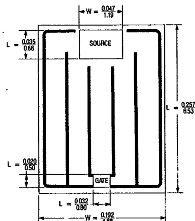
HEX-4.5: 500V, N-CHANNEL
