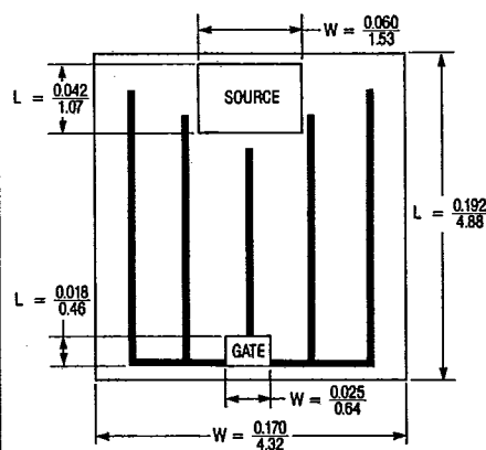
HEX-4: -100V, P-CHANNEL
