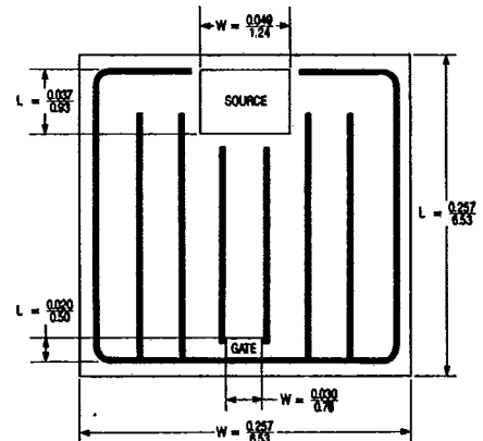
HEX-5: 400V, 500V, & 600V, N-CHANNEL
