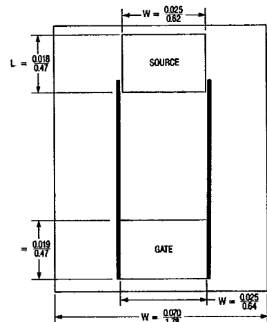
HEX-1: -100V, P-CHANNEL
