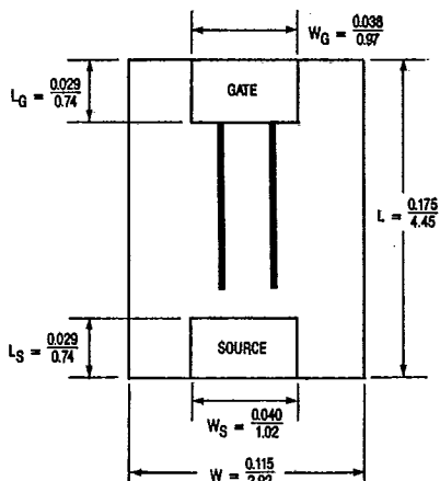
HEX-3: -200V, P-CHANNEL GEN I
