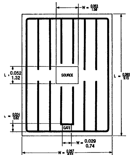
HEX-6: 200V, 400V & 500V N-CHANNEL
