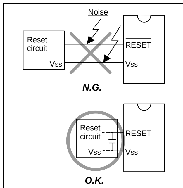
Fig 74. Wiring for the \overline{\text{RESET}} input pin
