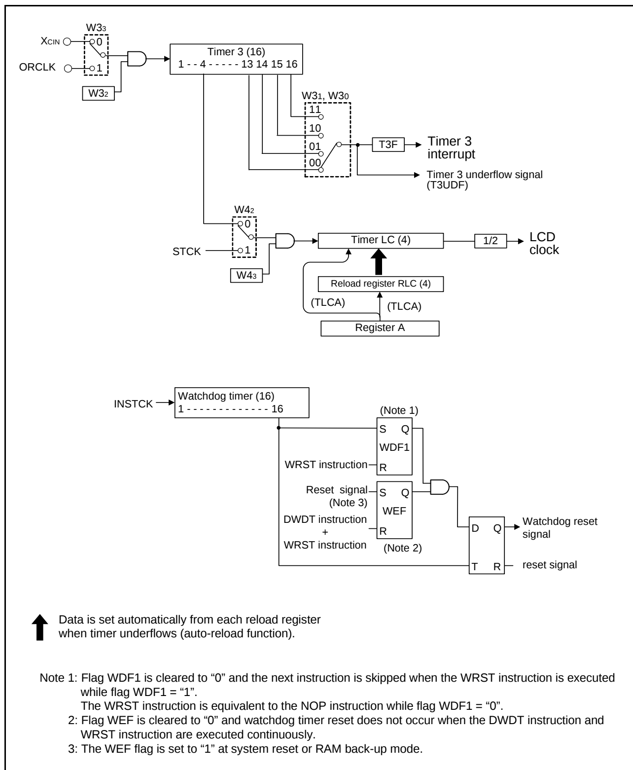
Fig 34. Timers structure (2)
