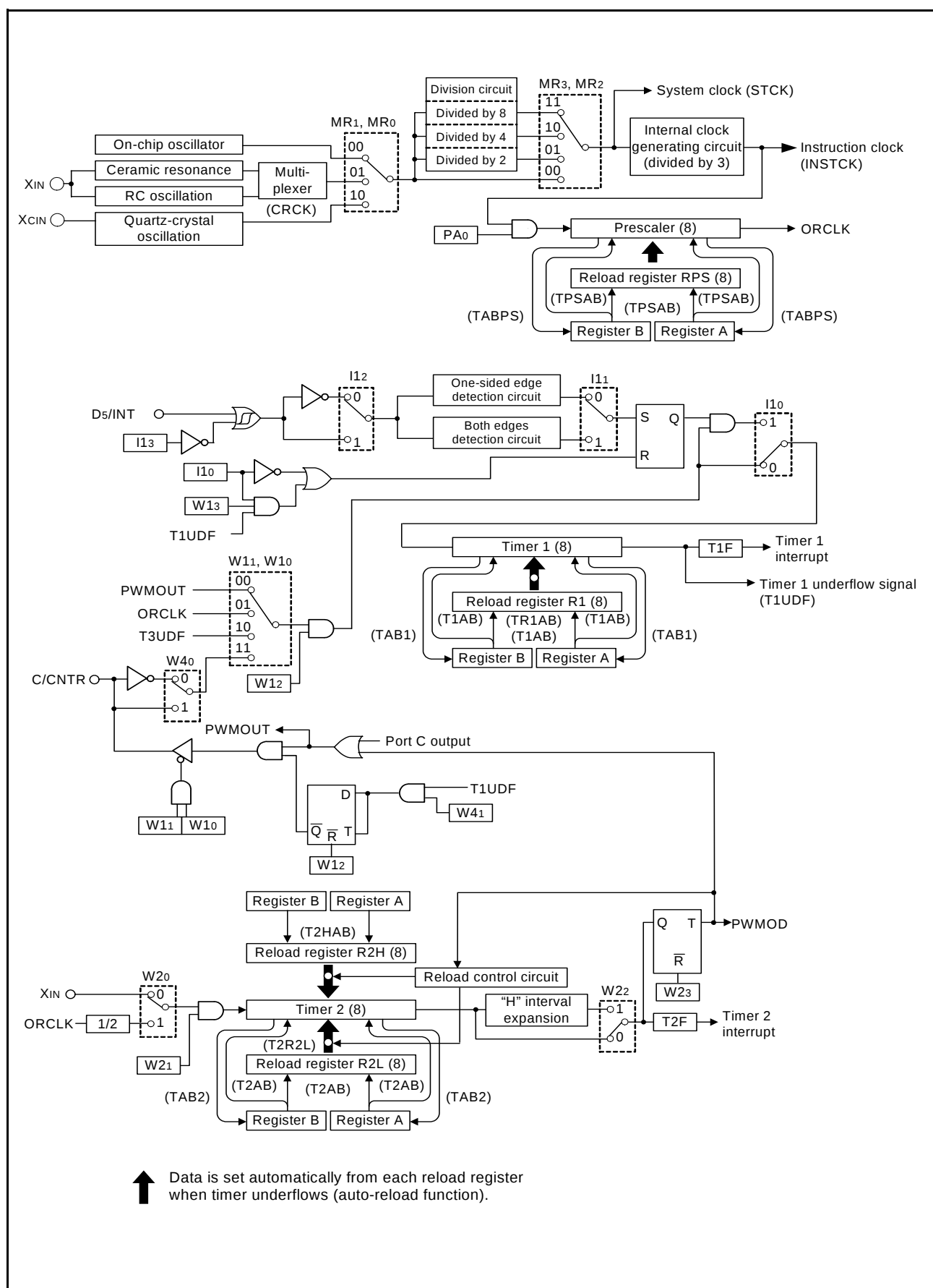
Fig 33. Timers structure (1)
