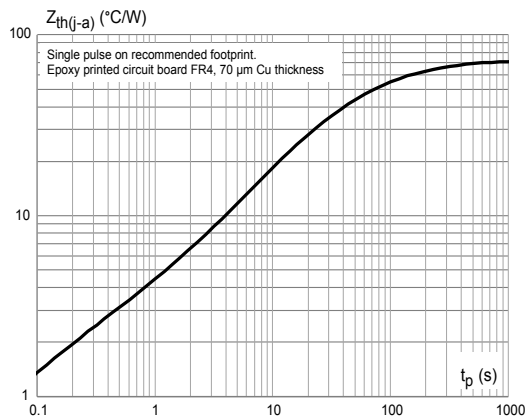
Figure 11. Thermal impedance junction to ambient versus pulse duration
