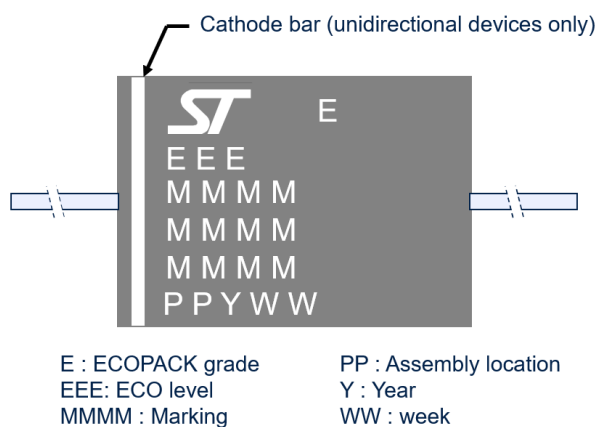
Figure 14. Marking layout
