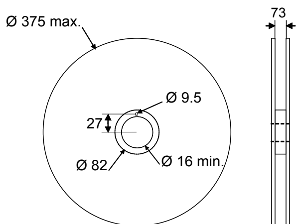
Figure 16. Reel dimension values (mm)
