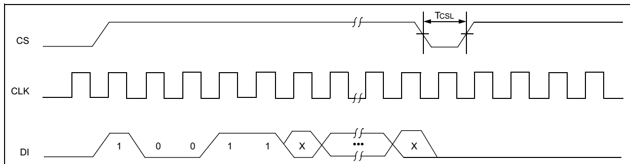
FIGURE 2-6: EWEN TIMING
