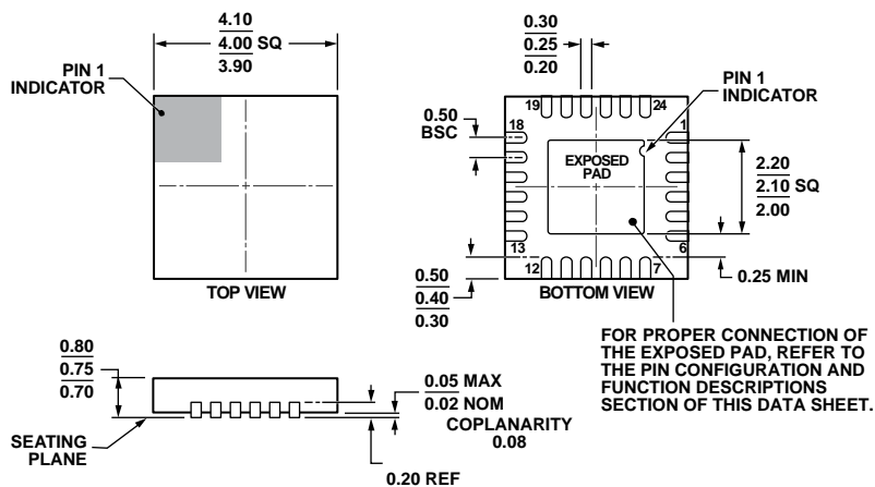
Figure 19. 24-Lead Lead Frame Chip Scale Package [LFCSP_WQ]
