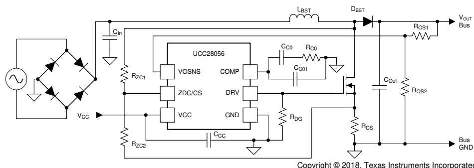
Simplified Application
