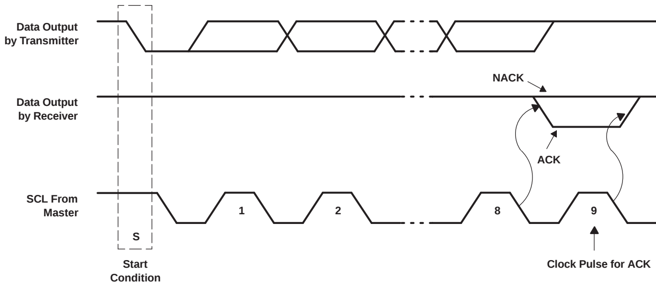
Figure 7. Acknowledgment on the I²C Bus
