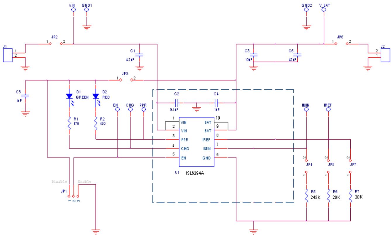
FIGURE 2. SCHEMATIC
