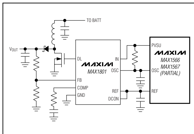
Figure 14. Adding a PWM Channel with an External MAX1801 Slave Controller
