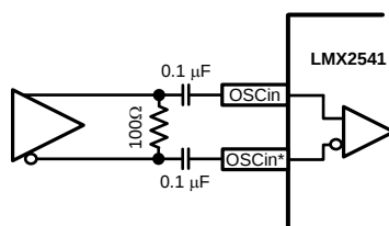
Figure 35. Differential Operation
