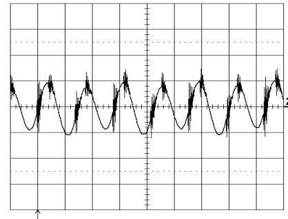
Output voltage ripple at: T_{ref} = +25^{\circ}\text{C} , V_I = 53\text{ V} , I_O = 20\text{ A} resistive load. Trace: output voltage (20 mV/div.). Time scale: (2 μs/div.).
