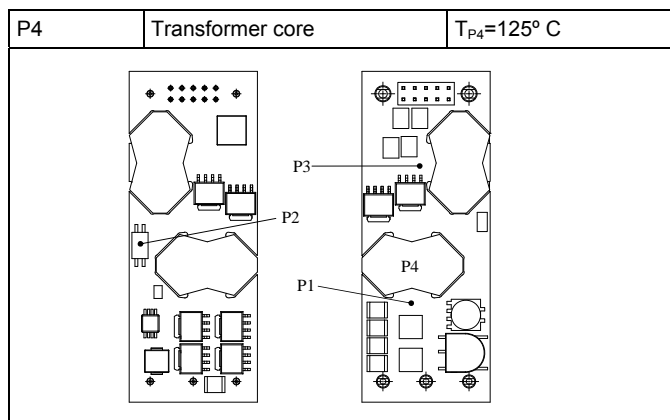
Top view Bottom view (Best airflow direction Negative to Positive.)
