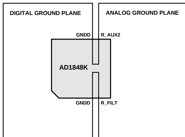
Figure 25. AD1848K Recommended Ground Plane
