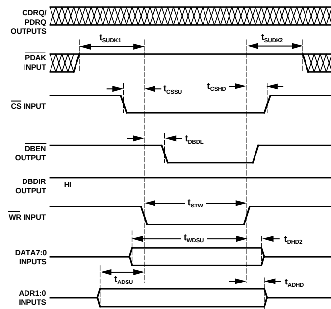
Figure 12. AD1848K Control Register/PIO Write Cycle
