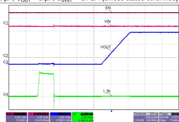
Figure 26. Transient: Recovery From Short Circuit / Over Current
