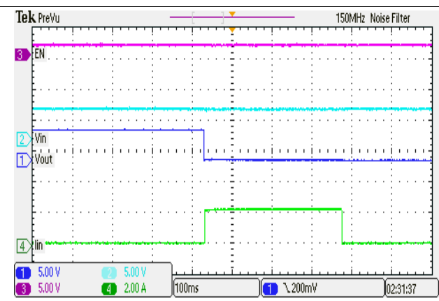
Figure 28. Transient: Overload Current Limit
