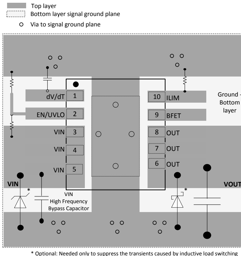
Figure 44. Layout Example
