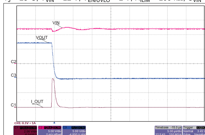
Figure 25. Short Circuit (Zoom): Fast-Trip Comparator
