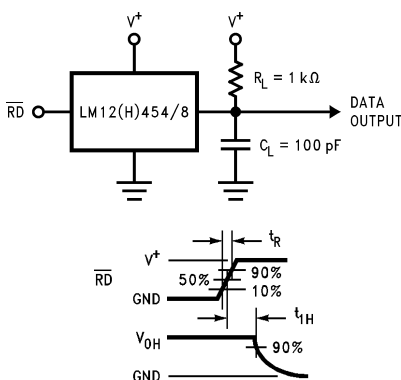
Figure 40. TRI-STATE Test Circuits and Waveforms
