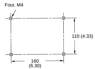
Mounting Holes
