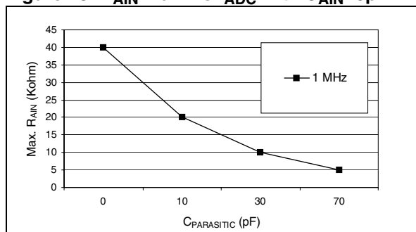
Figure 78. R_{AIN} max. vs f_{ADC} with C_{AIN}=0\text{pF} 3)
