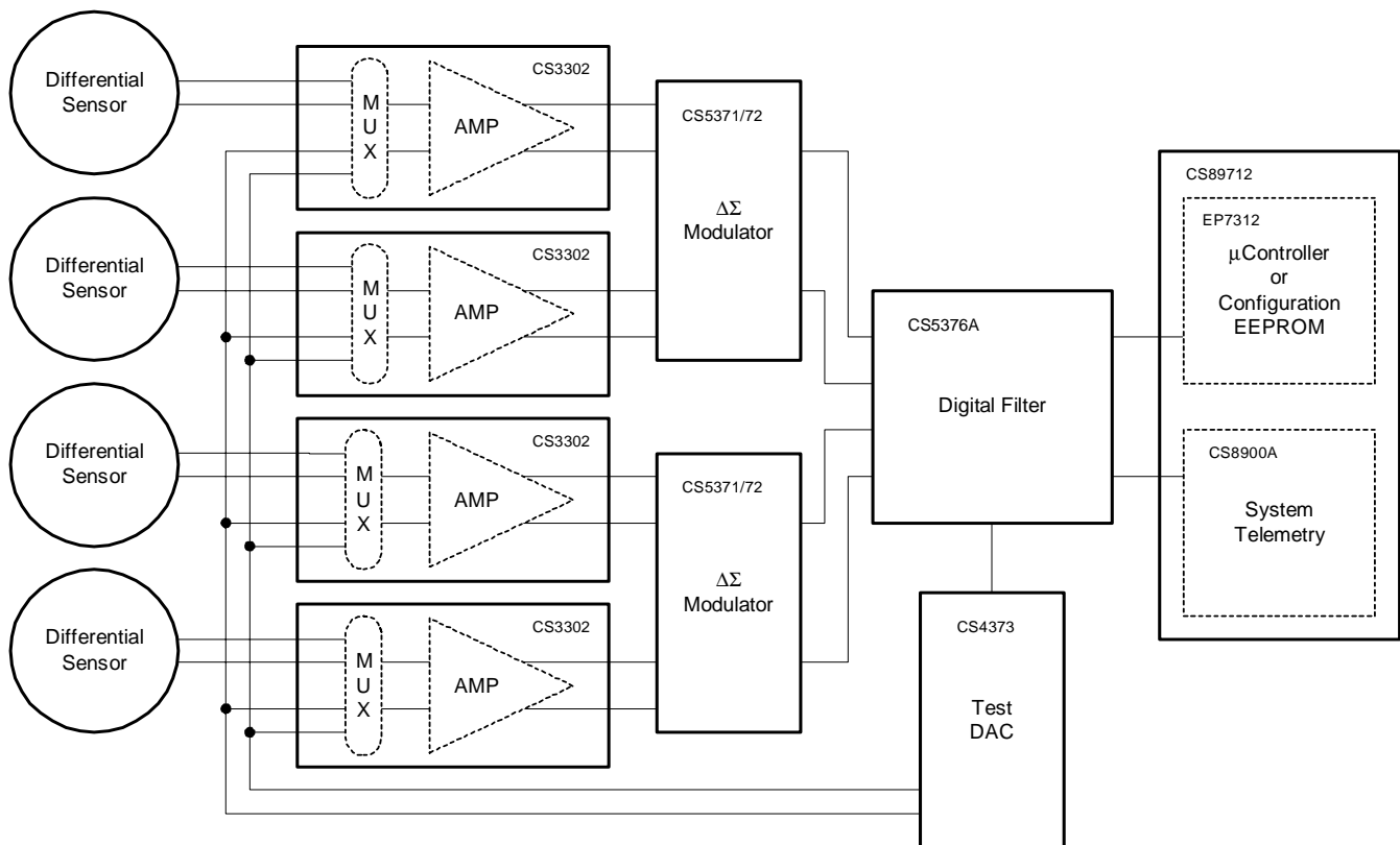
Figure 3. System Architecture
