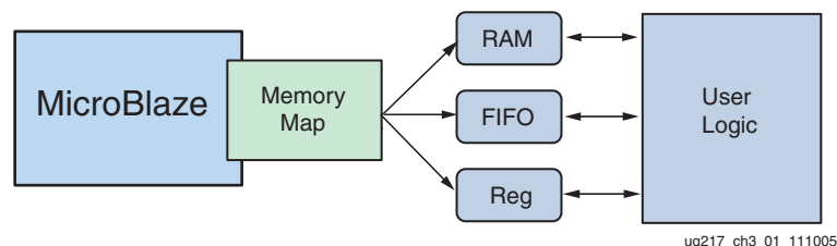
Figure 3-1: Memory-Mapped User Logic
