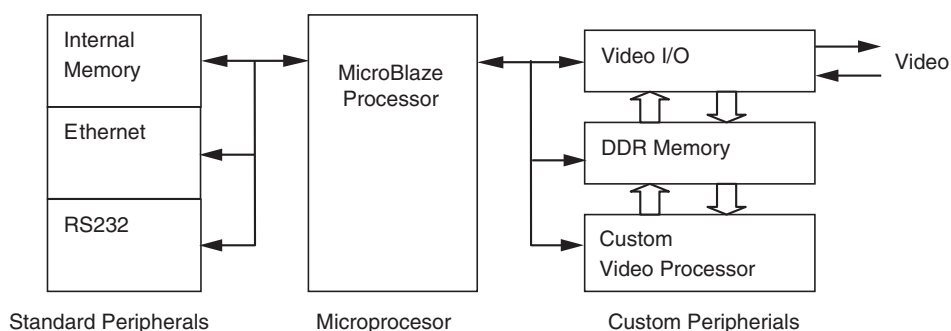
Figure 2-7: MicroBlaze Processor with Peripherals and Three Custom Video Peripherals
