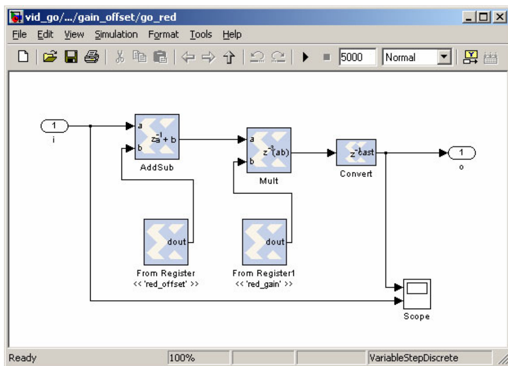
Figure 6-5: Connecting the Blocks
