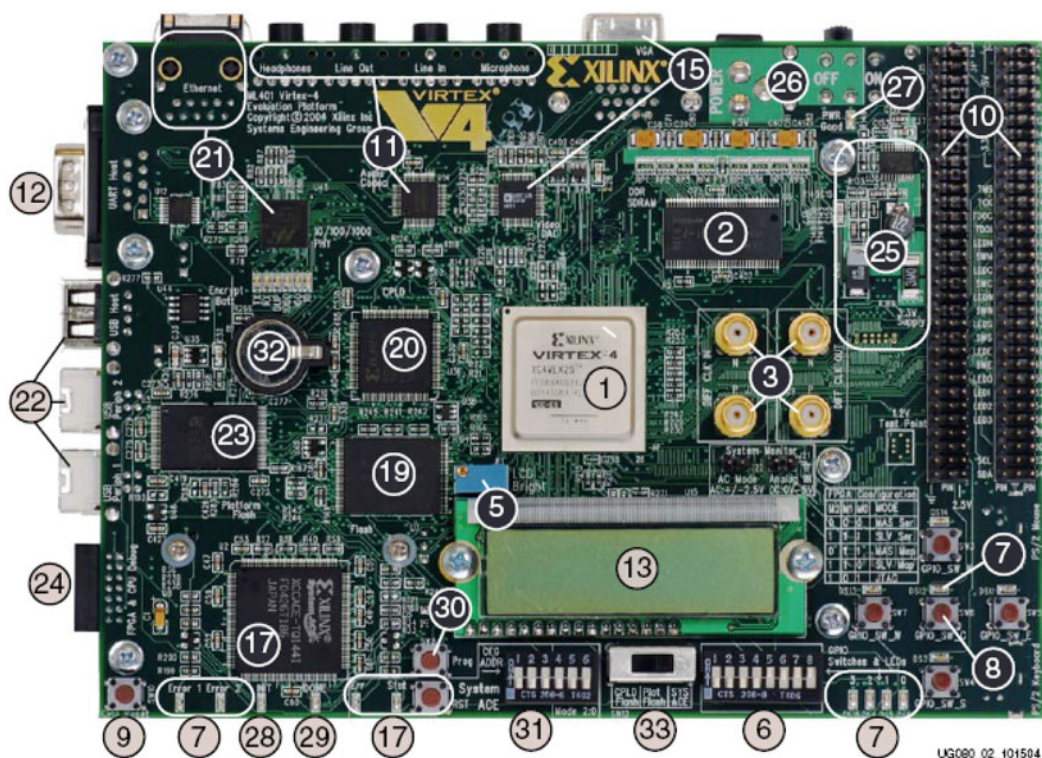
Figure A-5: ML402 Board
