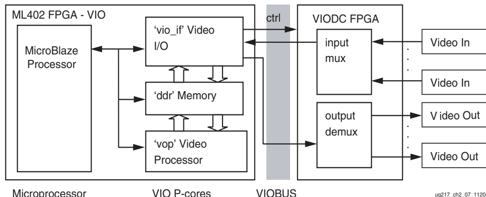
Figure 2-11: ML402 FPGA
