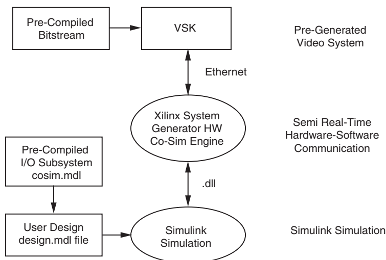
Figure 1-8: Hardware-in-the-Loop Flow
