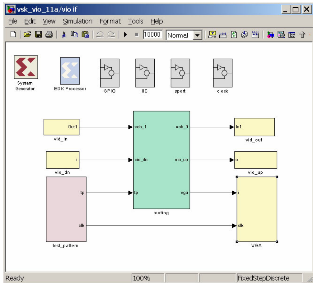
Figure 5-10: VIO Pcore Top-Level Diagram
