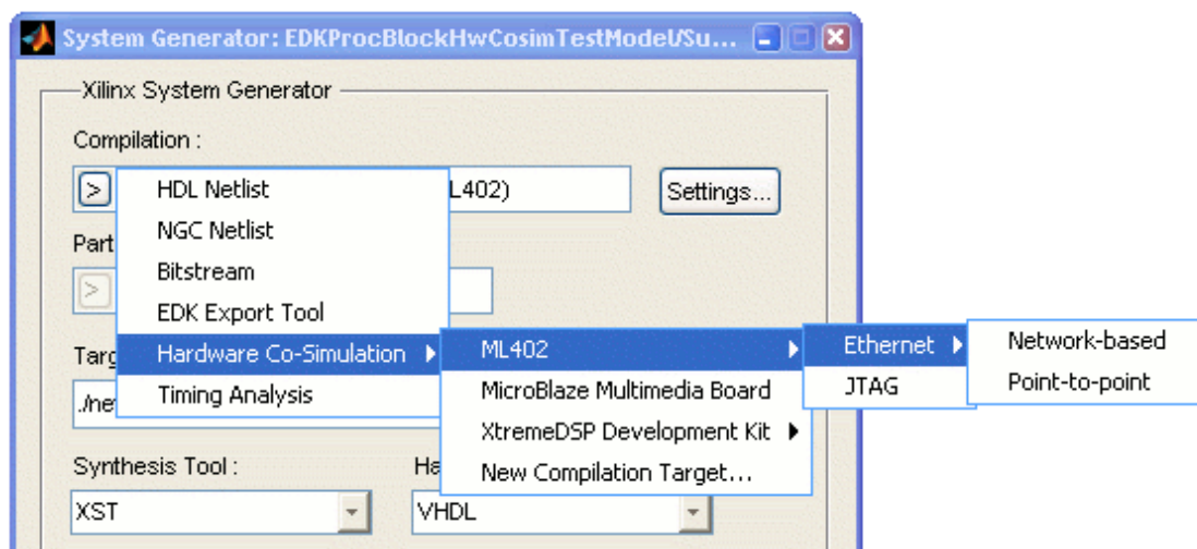
Figure 3-7: Hardware Co-Simulation Options
