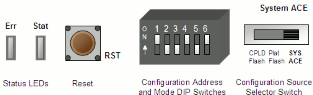
Figure 4-13: On-Board Settings
