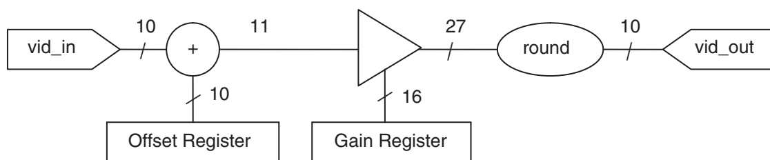
Figure 6-1: Gain and Offset
