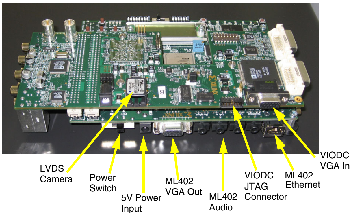
Figure A-1: VIODC Rear View
