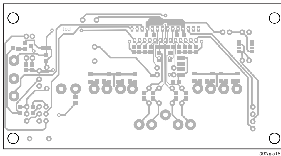
Fig 34. PCB layout of test and application circuit; copper layer bottom (top view)
