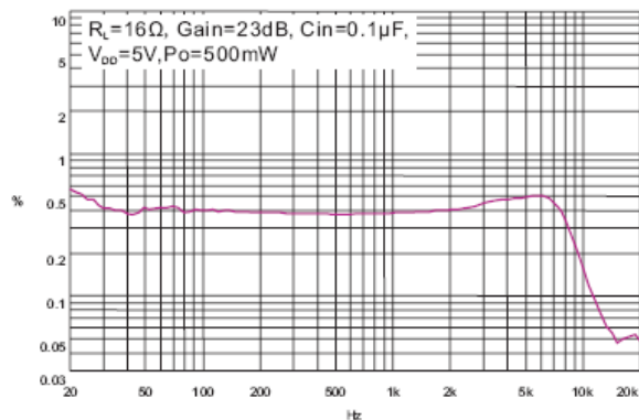
8. THD+N VS Frequency
