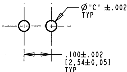
RECOMMENDED HOLE PATTERN GAUGE
