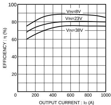
Fig.11 Efficiency
