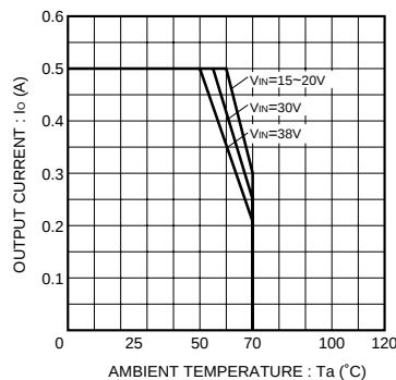
Fig.16 Derating curve
