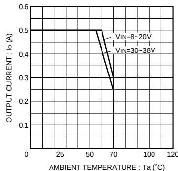
Fig.13 Derating curve
