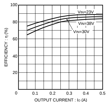
Fig.17 Efficiency
