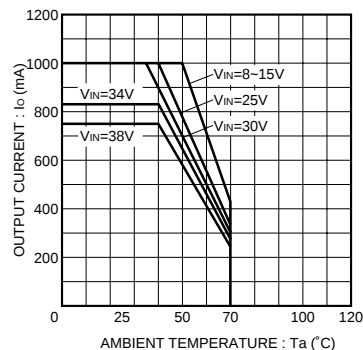
Fig.10 Derating curve
