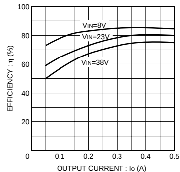
Fig.14 Efficiency
