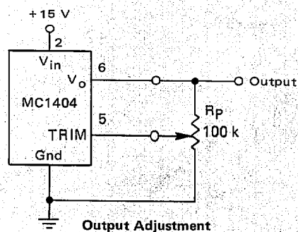
FIGURE 10 — OUTPUT TRIM CONFIGURATION
