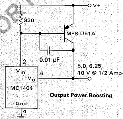
FIGURE 11 — PRECISION SUPPLY USING MC1404
