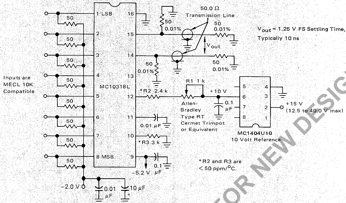
FIGURE 14 — HIGH SPEED 8-BIT D/A CONVERTER USING MC1404U10
