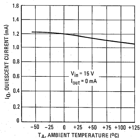
FIGURE 7 – QUIESCENT CURRENT versus TEMPERATURE
