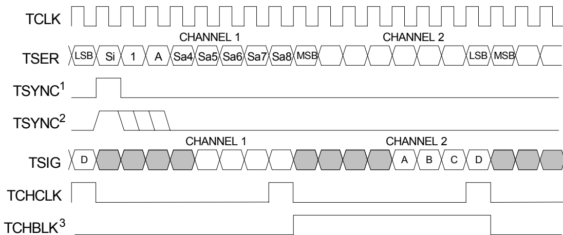
Figure 13-20. E1 Transmit-Side Boundary Timing (Elastic Store Disabled)
