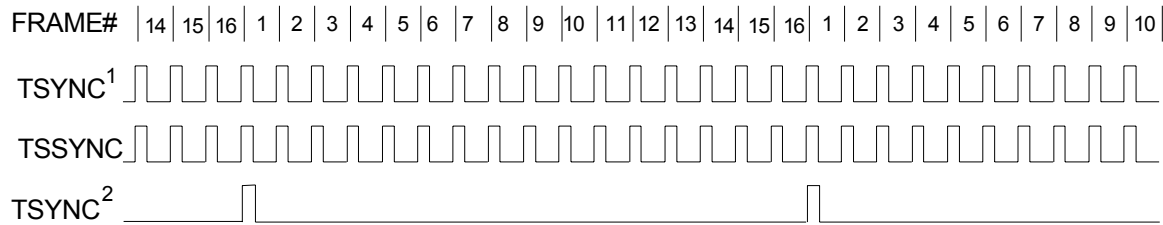
Figure 13-19. E1 Transmit-Side Timing
