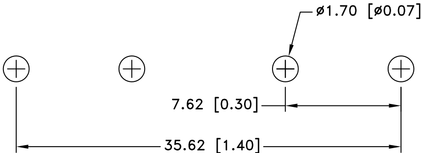
MOUNTING DETAIL
