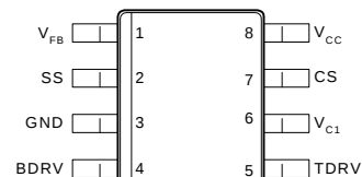
LX1682 DM PACKAGE (Top View)
