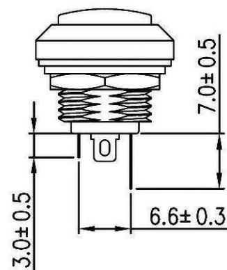
Illuminated Switch
