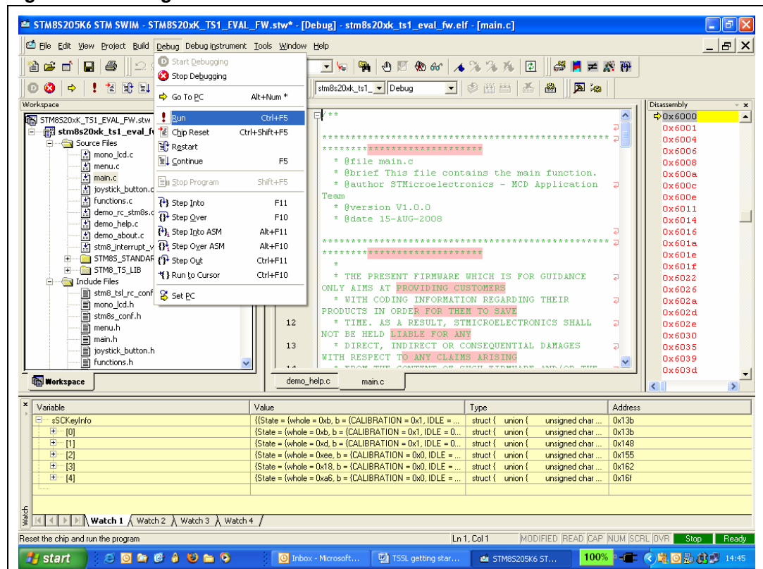
Figure 14. Debug mode
