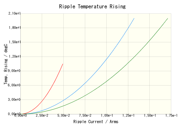
C1608X7R2A222K080AA(100kHz) C1608X7R2A222K080AA(500kHz) C1608X7R2A222K080AA(1MHz)
