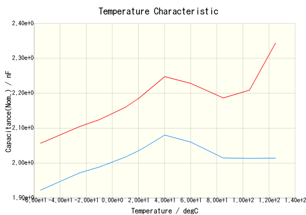
C1608X7R2A222K080AA(DC Bias = 0V) C1608X7R2A222K080AA(DC Bias = 50V)
