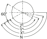
Keyway Positions, Shell Size 7-12
