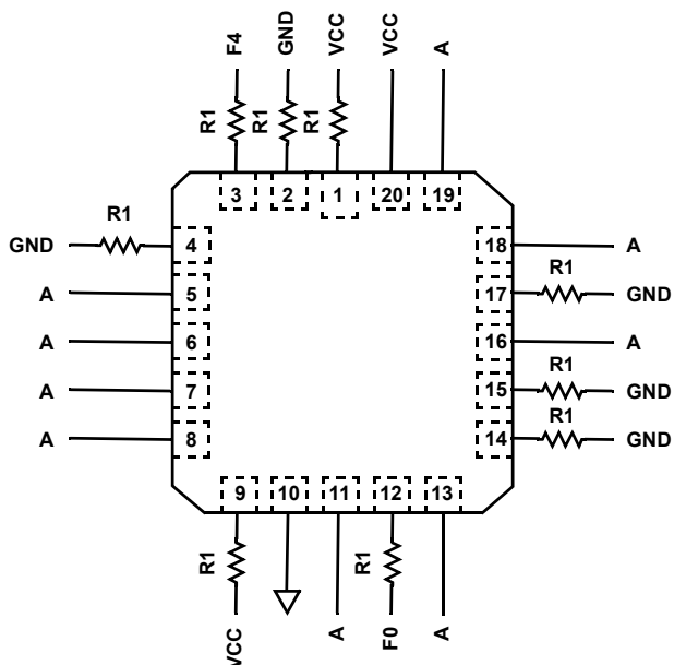
HD-6409/883 CLCC
