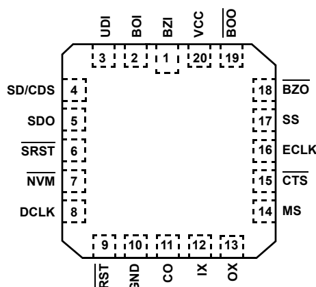
HD4-6409/883 (CLCC) TOP VIEW
