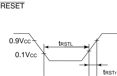
Figure 106 Reset Timing
