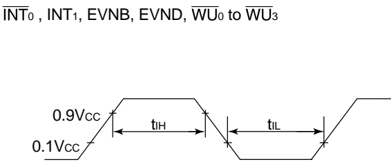
Figure 105 Interrupt Timing
