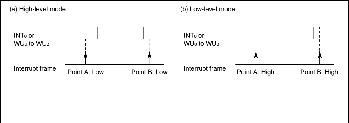
Figure 21 Sampling Examples
