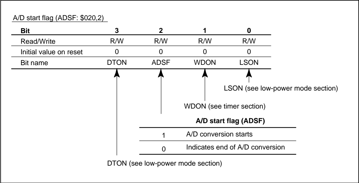
Figure 81 A/D Start Flag (ADSF)
