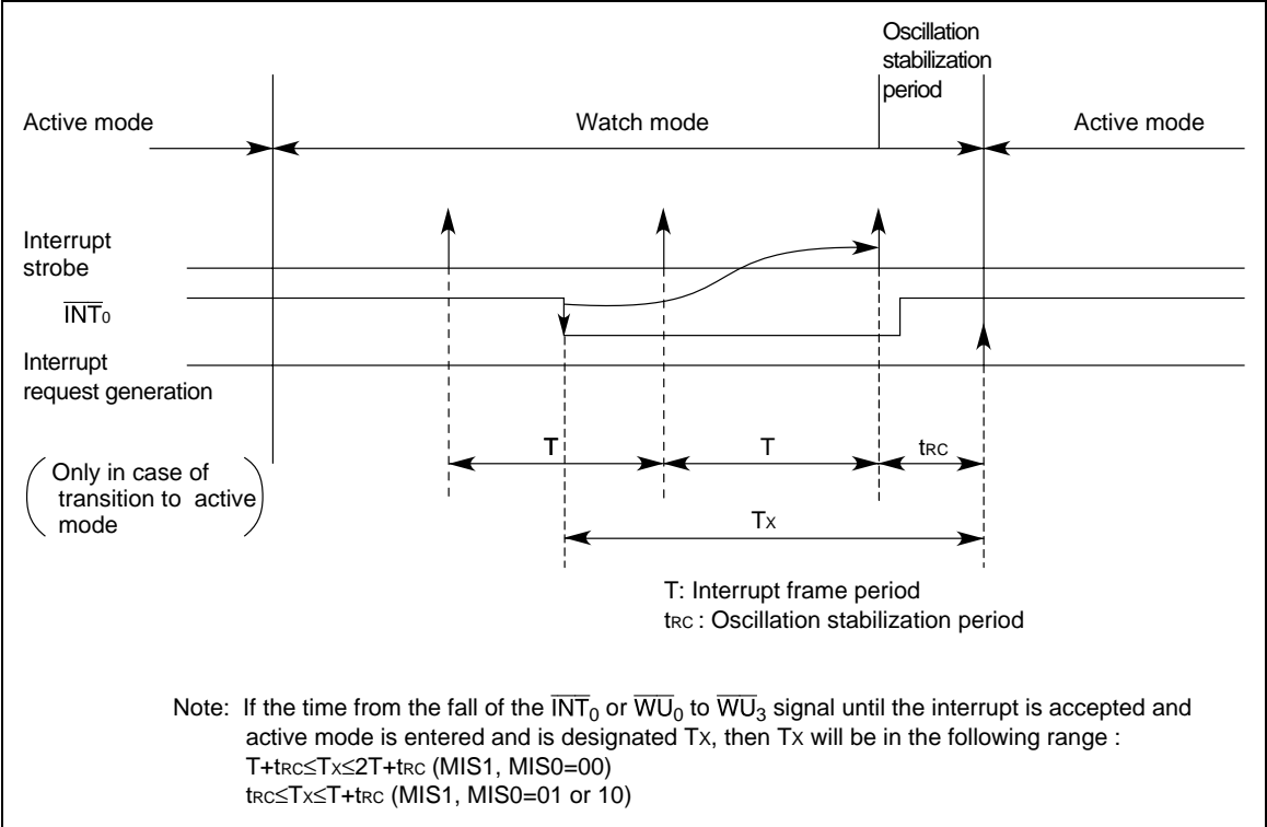
Figure 16 Interrupt Frame
