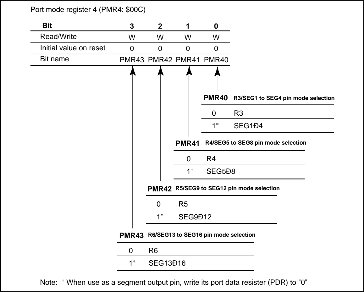
Figure 90 Port Mode Register 4 (PMR4: $00C)
