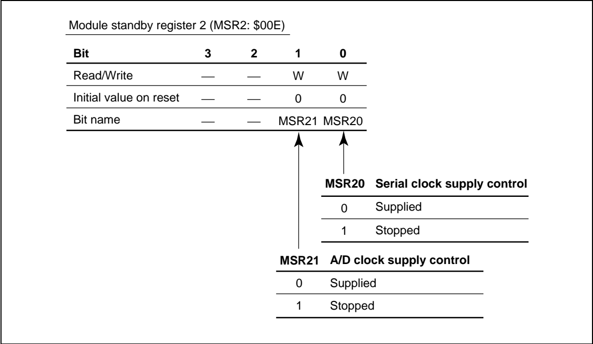
Figure 72 Module Standby Register 2 (MSR2)
