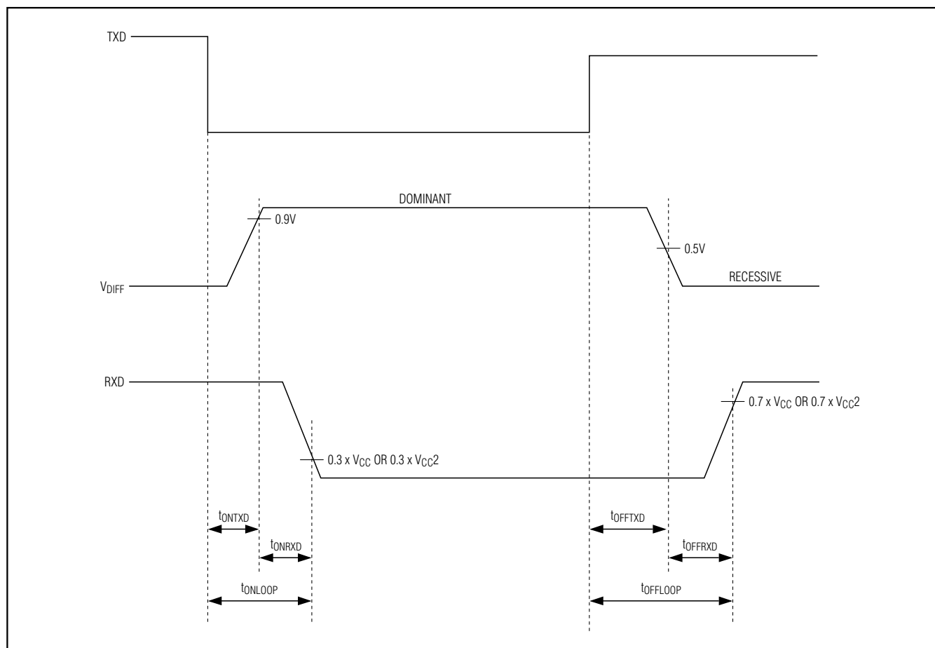
Figure 1. Timing Diagram
