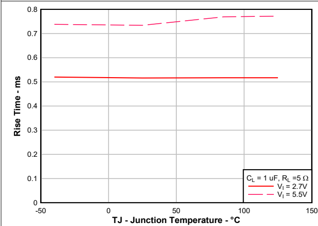
Figure 6-3. Rise Time vs Junction Temperature
