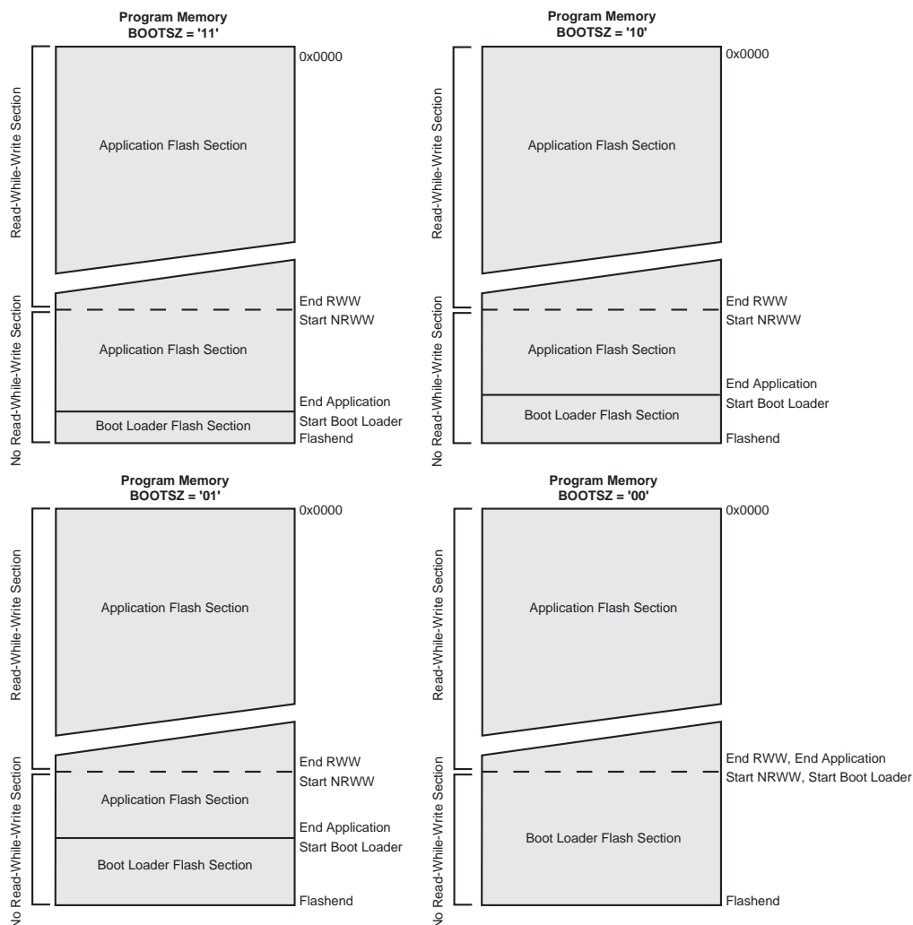
Figure 116. Memory Sections
