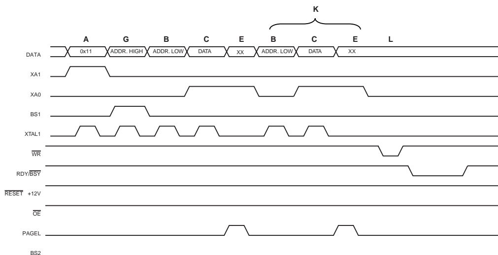
Figure 121. Programming the EEPROM Waveforms
