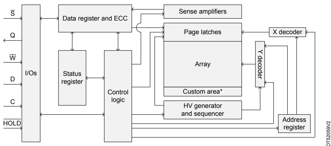
Figure 4. Block diagram
