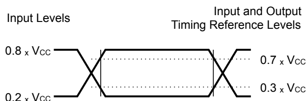
Figure 19. AC measurement I/O waveform
