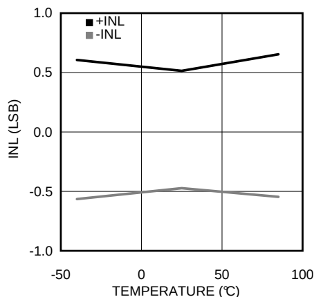
Figure 4-10. INL vs. Temperature (ADC12D1800RF)
