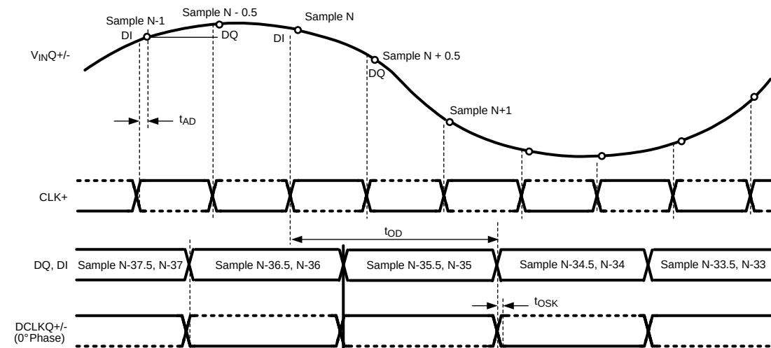
Figure 4-4. Clocking in 1:4 Demux DES Mode*
