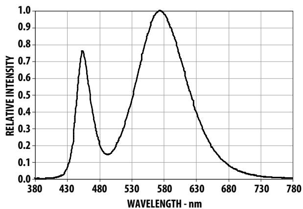
Figure 3. Relative Intensity vs. Wavelength for Neutral White
