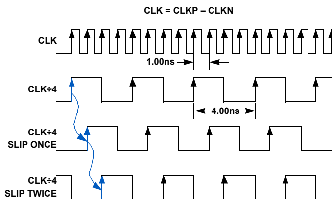
FIGURE 42. PHASE SLIP: CLK÷4 MODE, f_{\text{CLK}} = 1000\text{MHz}
