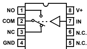
ISL84544 (SOIC) TOP VIEW
