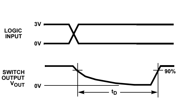
FIGURE 2C. MEASUREMENT POINTS (ISL84544 ONLY)
