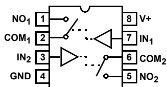
ISL84541 (SOIC) TOP VIEW
