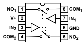
ISL84541 (SOT-23) TOP VIEW
