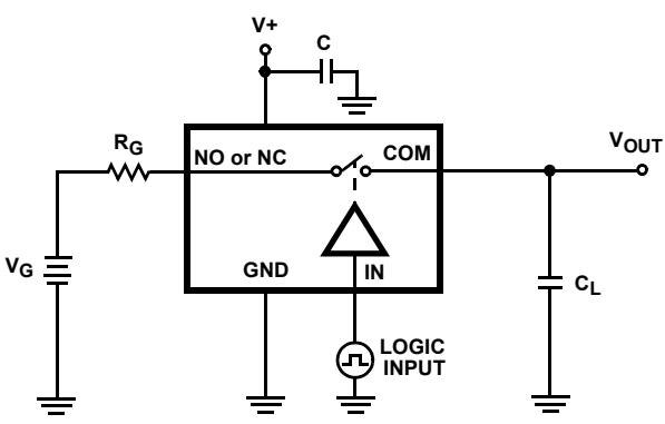
FIGURE 2B. TEST CIRCUIT
