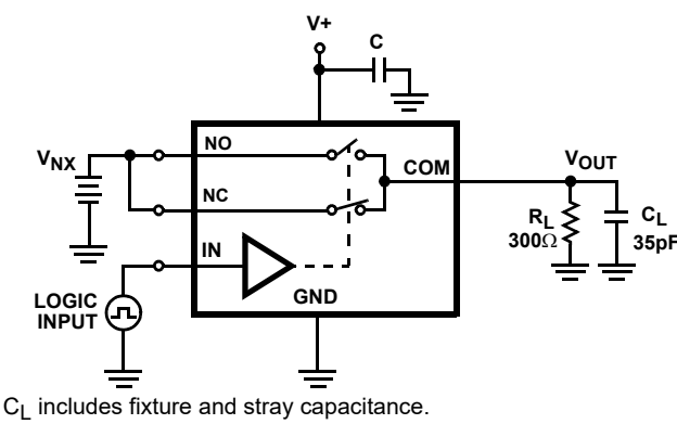
FIGURE 2D. TEST CIRCUIT (ISL84544 ONLY)
