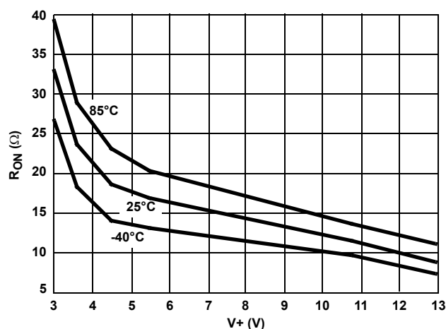
FIGURE 8. ON-RESISTANCE vs SUPPLY VOLTAGE
