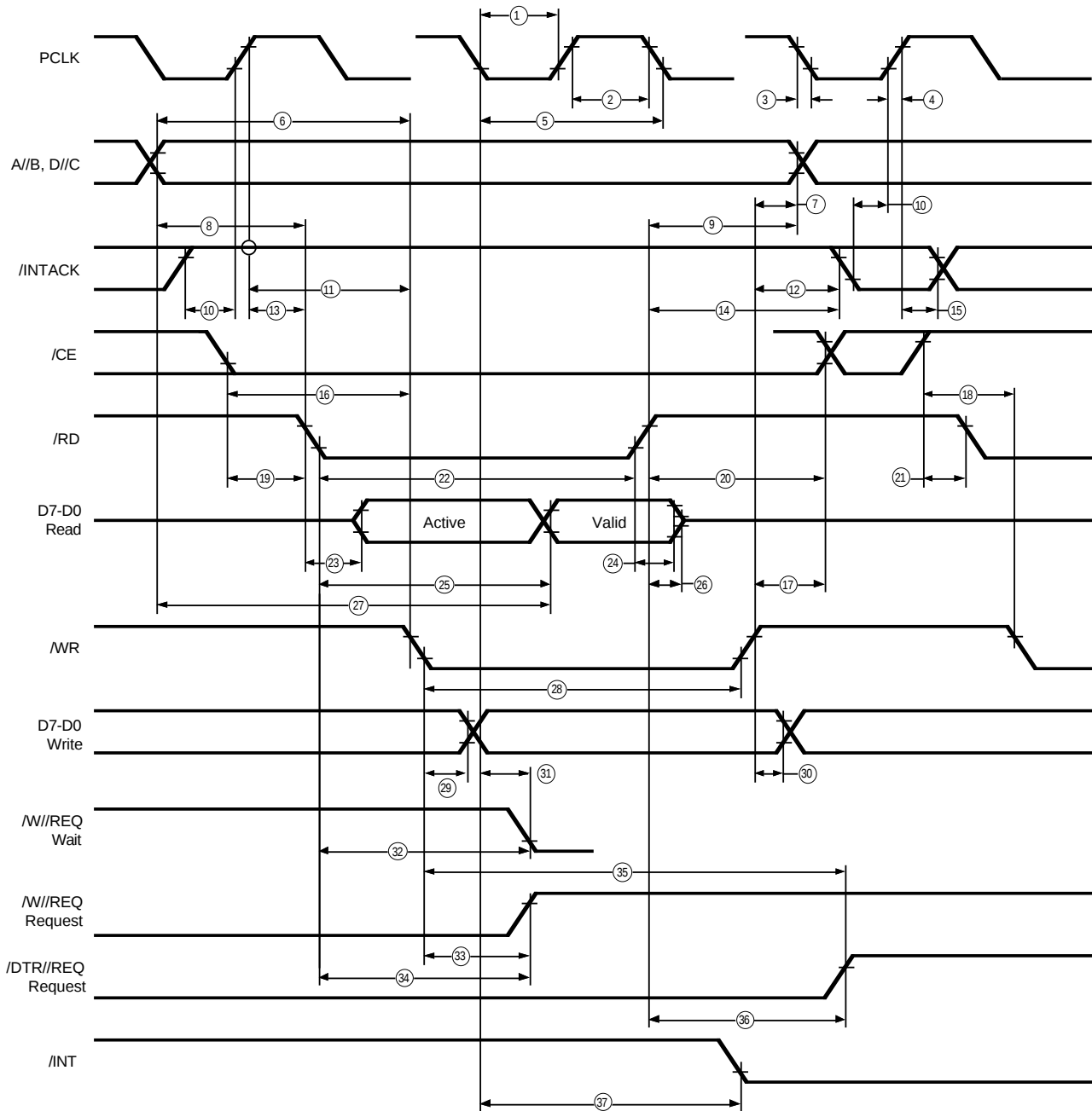
Read and Write Timing Diagram
