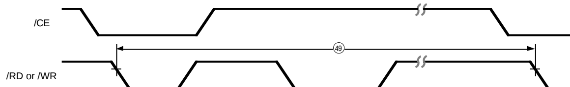
Cycle Timing Diagram
